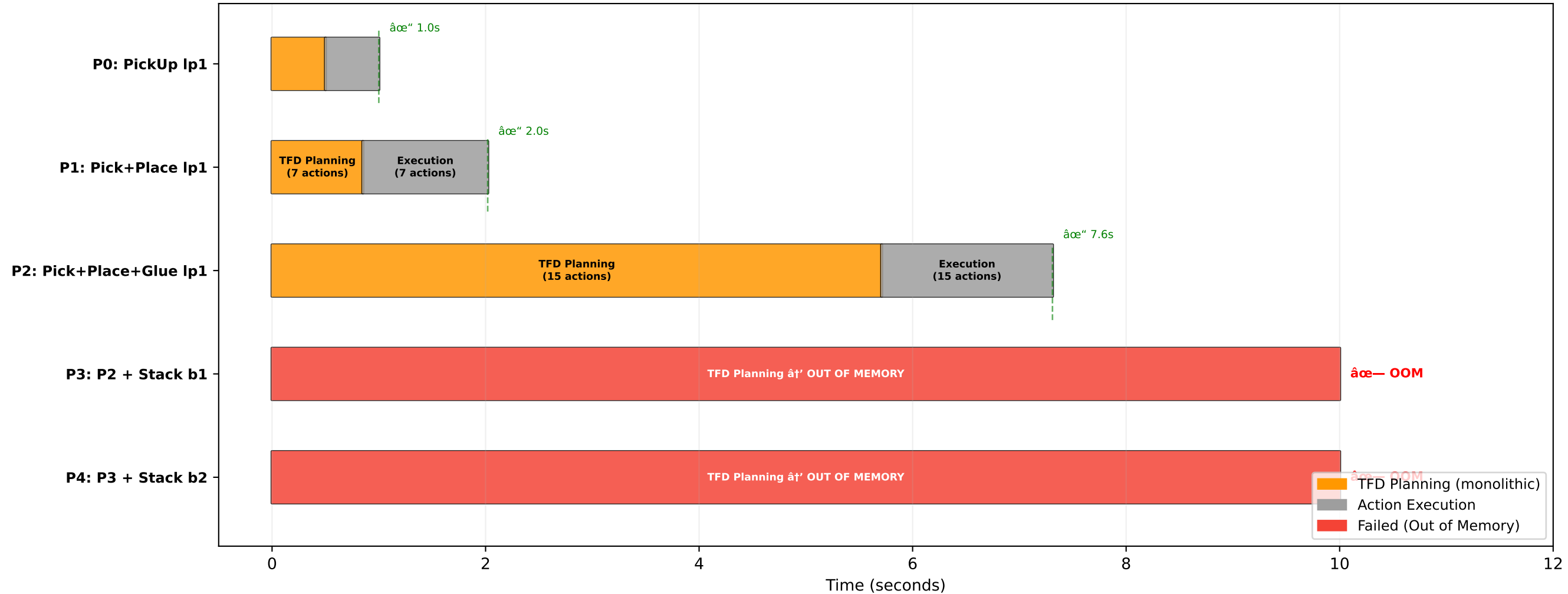
PlanSys2 Monolithic Planning: Execution Timeline for Increasing Problem Complexity (Each row = one run; TFD planning in orange, execution in grey, failure in red)
